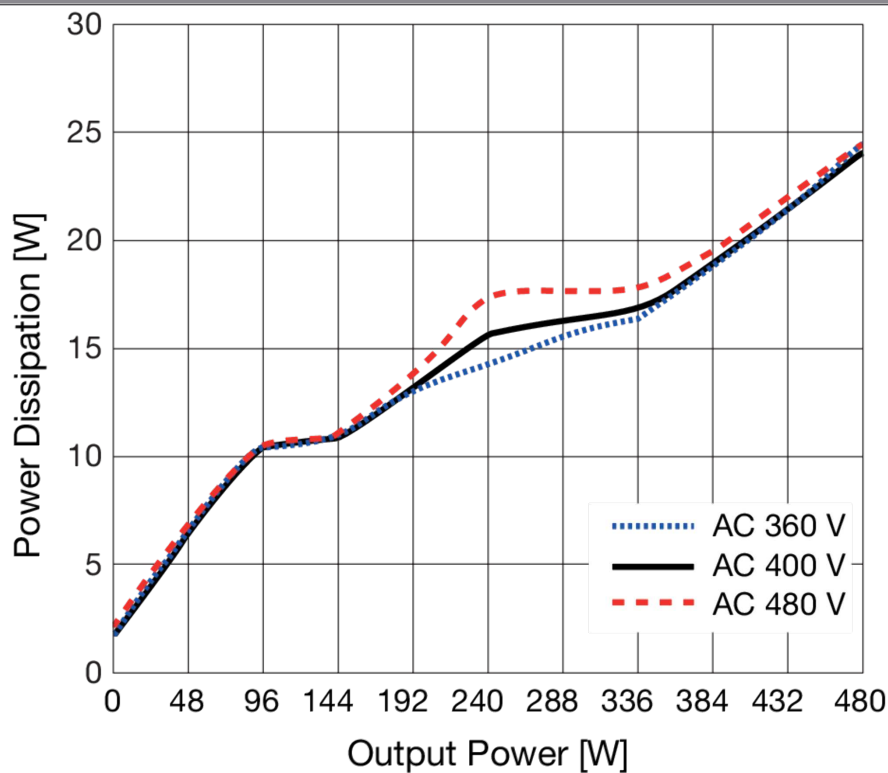
POWER DISSIPATION VS. LOAD 480 W DC 24 V
