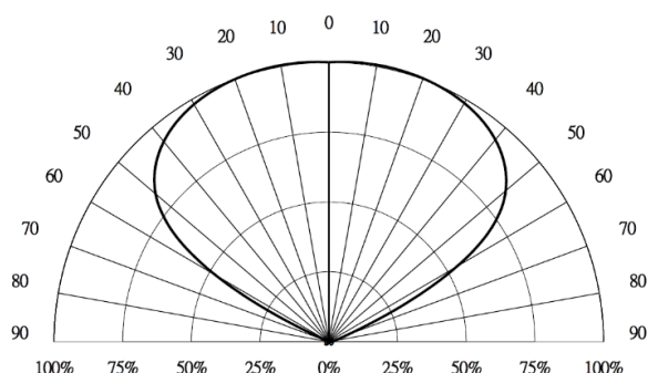
Radiation Diagram
