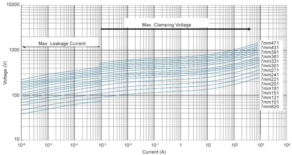
Voltage Curve - 7 mm 820K-471K
