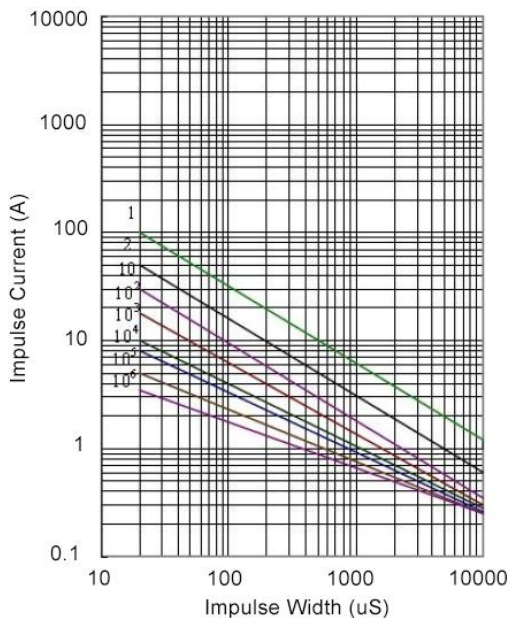
7 mm 180K - 680K
