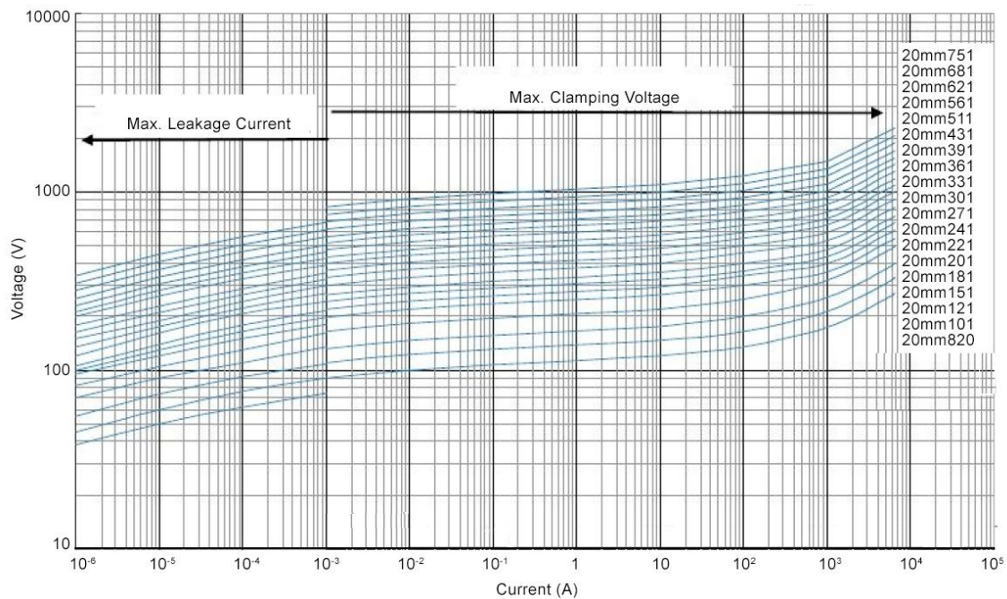
Voltage Curve - 20 mm 820K-751K
