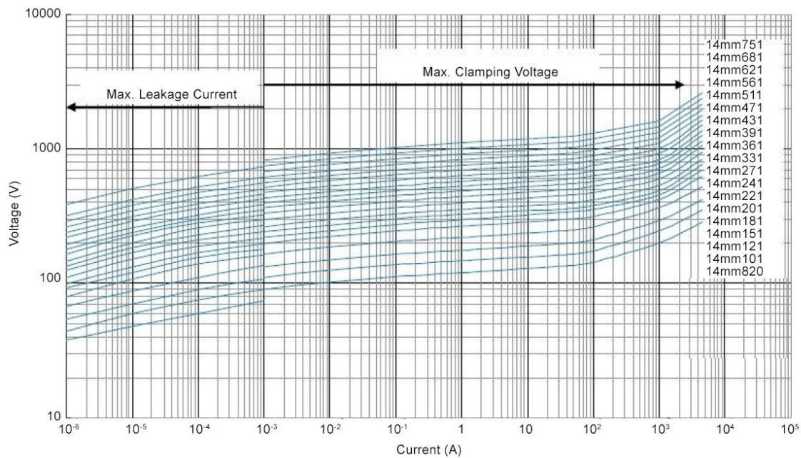
Voltage Curve - 14 mm 820K-751K
