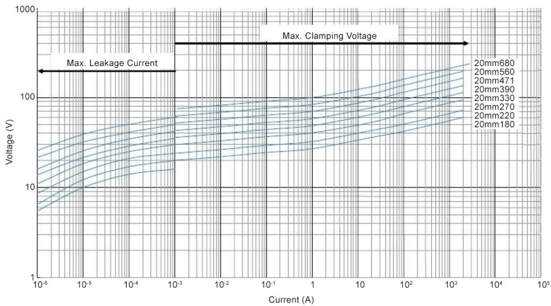
Voltage Curve - 20 mm 180K-680K
