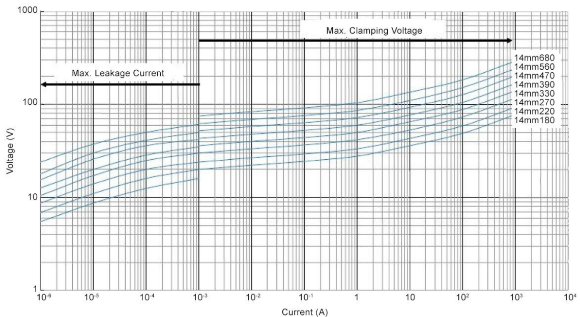
Voltage Curve - 14 mm 180L-680K
