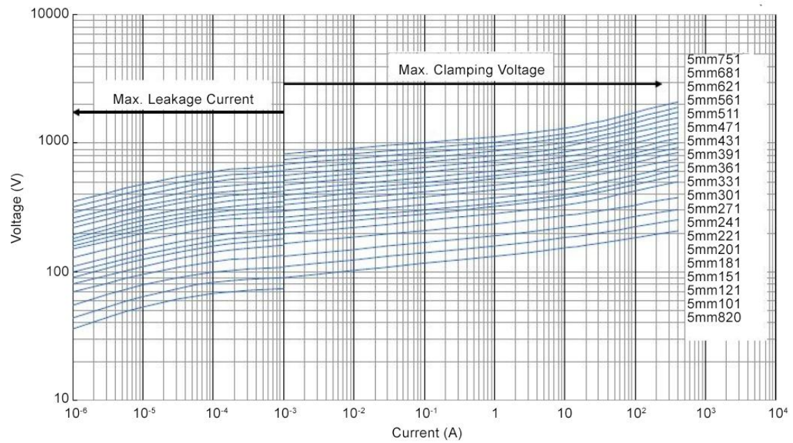
Voltage Curve - 5 mm 820K-751K
