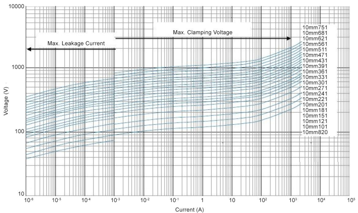
Voltage Curve - 10 mm 820K-751K
