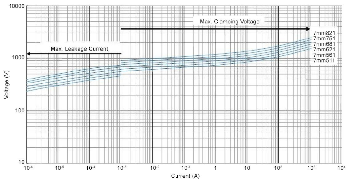
Voltage Curve - 7 mm 511K-821K
