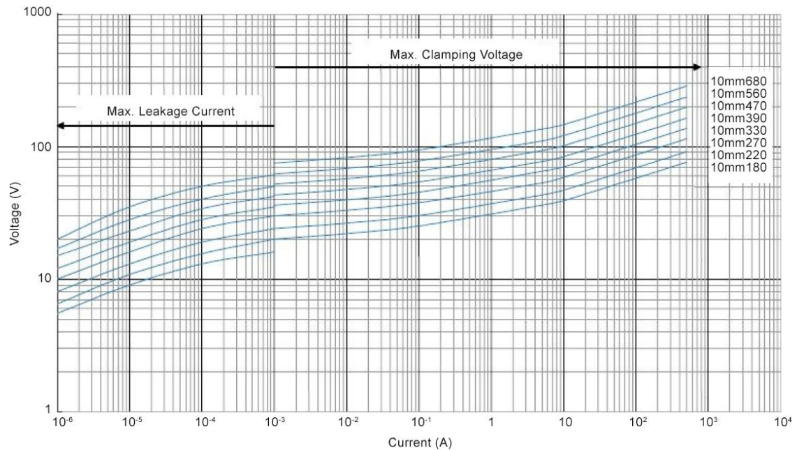
Voltage Curve - 10 mm 180L-680K
