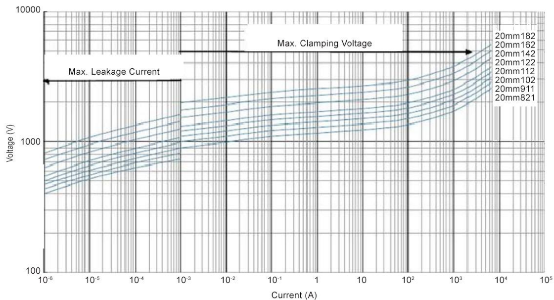
Voltage Curve - 20 mm 821K-182K
