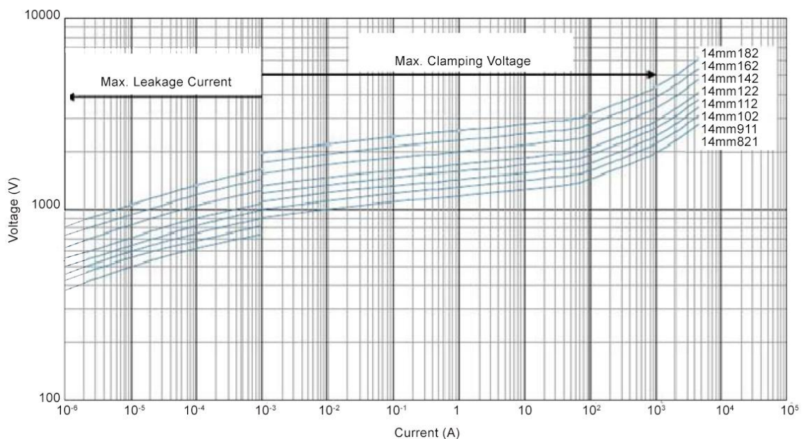
Voltage Curve - 14 mm 821K-182K
