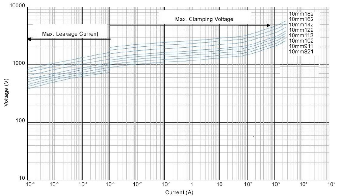
Voltage Curve - 10 mm 821K-182K
