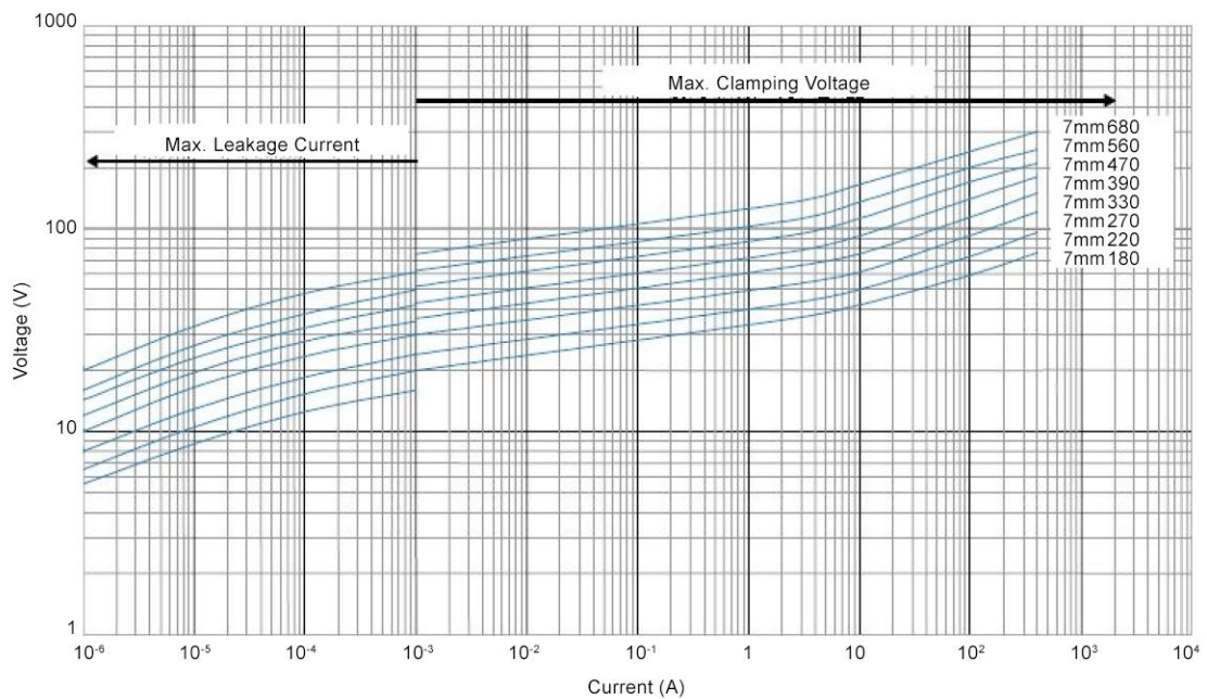
Voltage Curve - 7 mm 180K-680K
