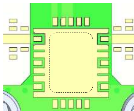
Mounting Detail Showing Copper Coin
