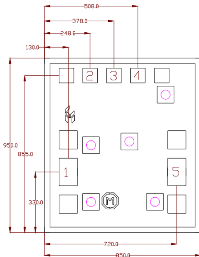
Die Outline (all dimensions in microns)
