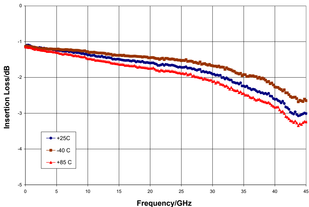
Insertion Loss versus Temperature
