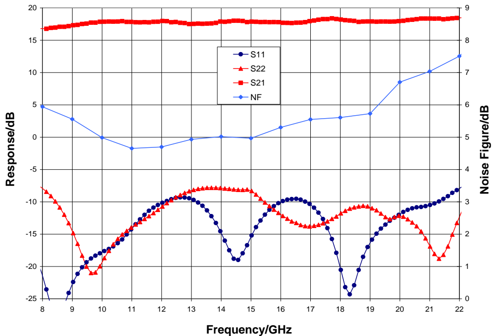
Narrow-band Performance, V_{dd} = 5.0 \text{ V} , V_{gg} = 3.0 \text{ V} , I_{dd} = 48 \text{ mA} , T_A = 25 \text{ }^\circ\text{C}
