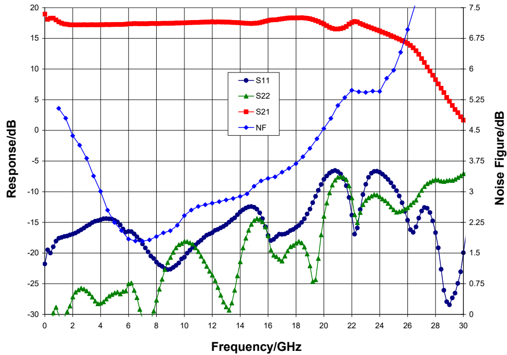
Broadband Performance, V_{dd} = 8.0\text{ V} , V_{gg} = -1.0\text{ V} , T_A = 25\text{ °C}
