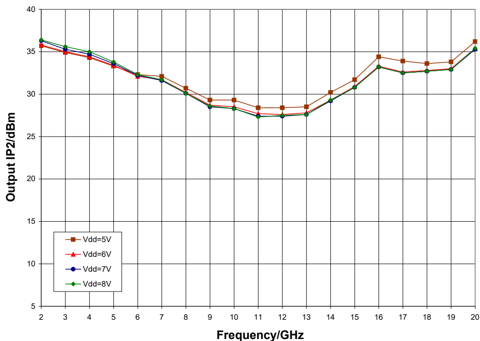
Output IP2 vs. V_{dd} , T_A = 25 \text{ °C}
