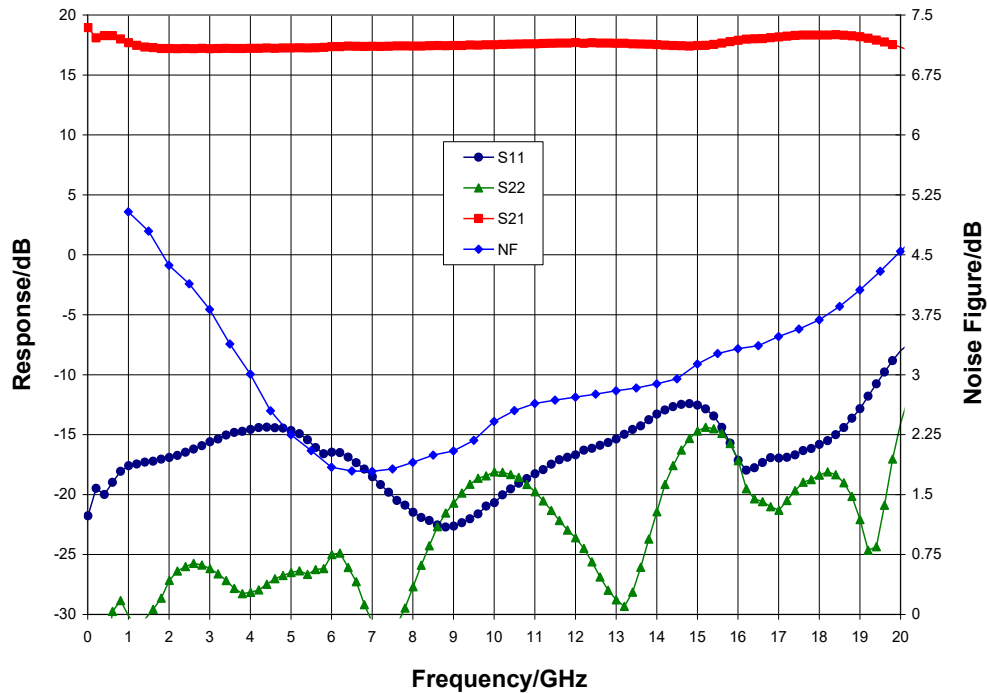
Narrow-band Performance, V_{dd} = 8.0\text{ V} , V_{gg} = -1.0\text{ V} , T_A = 25\text{ °C}
