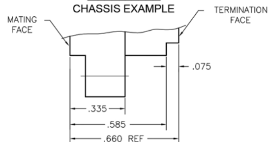
DETAIL A
