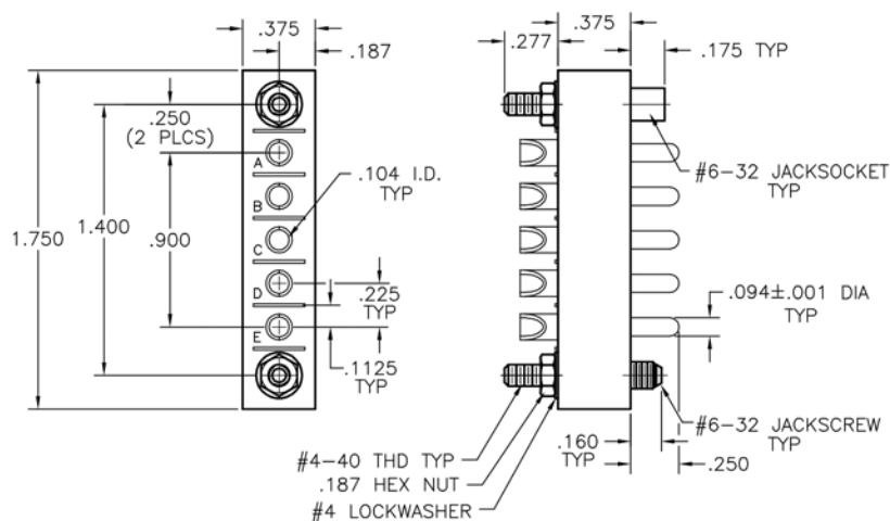
PLUG EXAMPLE: PA5PJ
