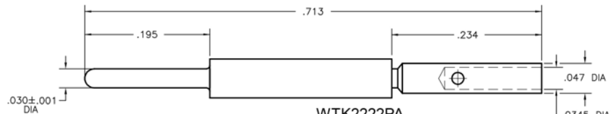
WTK2222PA PIN, CRIMP REMOVABLE, 22 GAGE BARREL
