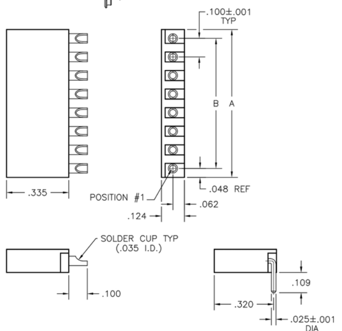
RIGHT ANGLE (WT8SAR7)
