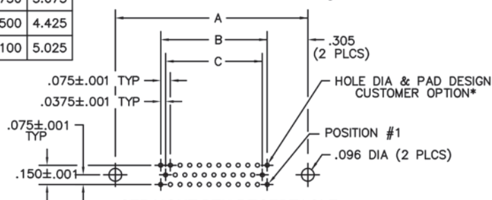
STRAIGHT PTH RECEPTACLE
