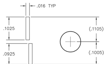
FOOTPRINT / PAD CONFIGURATION
