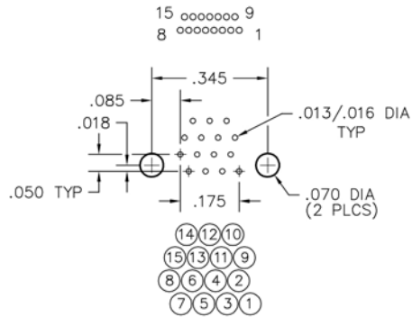
CONNECTOR MATING FACE
