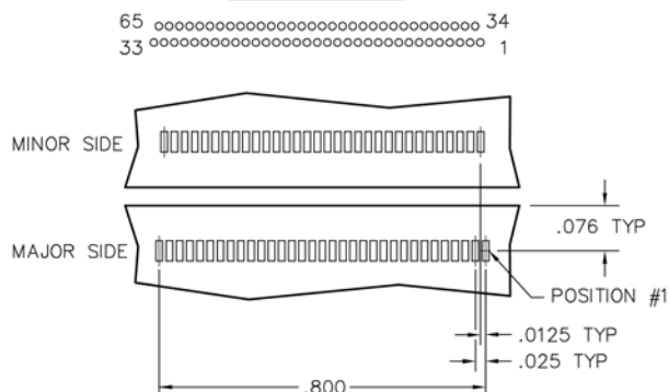
CONNECTOR MATING FACE
