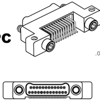
CONNECTOR MATING FACE
