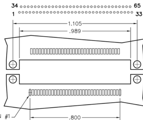
CONNECTOR MATING FACE
