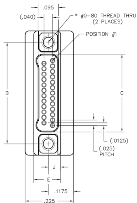
NK-2G2-025-135-TH00 PLUG
