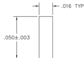
FOOTPRINT / PAD CONFIGURATION 15 POSITION
