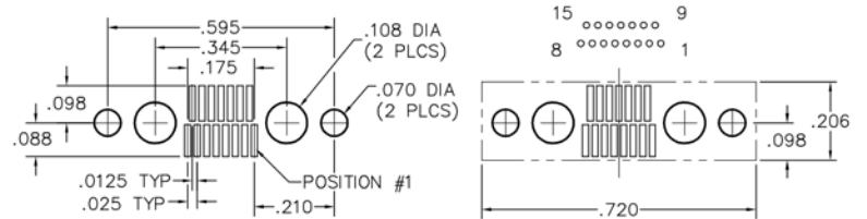
FOOTPRINT / PAD CONFIGURATION * = For .040" lead envelope, add .020" to noted dimensions
