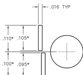
FOOTPRINT / PAD CONFIGURATION
