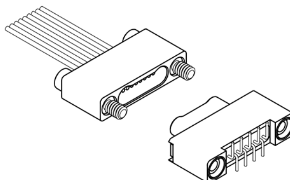
Cable to Vertical SMT Sizes: 9 thru 51 Page: N-23 & N-25
