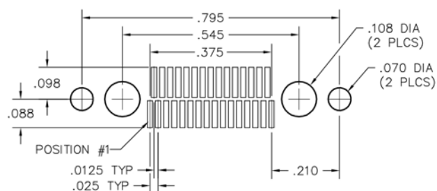
FOOTPRINT / PAD CONFIGURATION * = For .040" lead envelope, add .020" to noted dimensions
