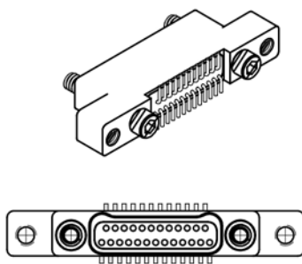
CONNECTOR MATING FACE
