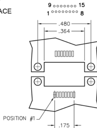
FOOTPRINT / PAD CONFIGURATION 15 POSITION
