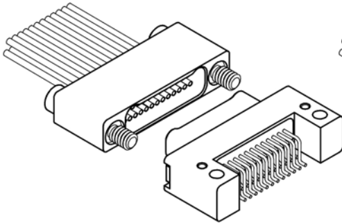
Cable to Horizontal SMT Sizes: 9 thru 91 Page: N-49 & N-51
