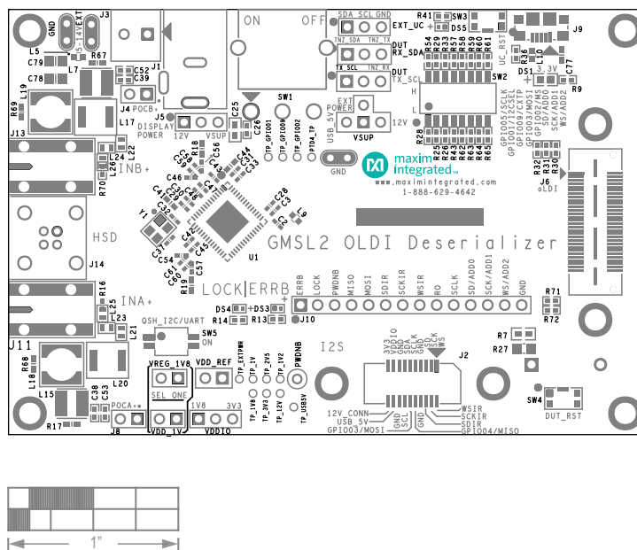
MAX96752 EV Kit Component Placement Guide—Top Silkscreen
