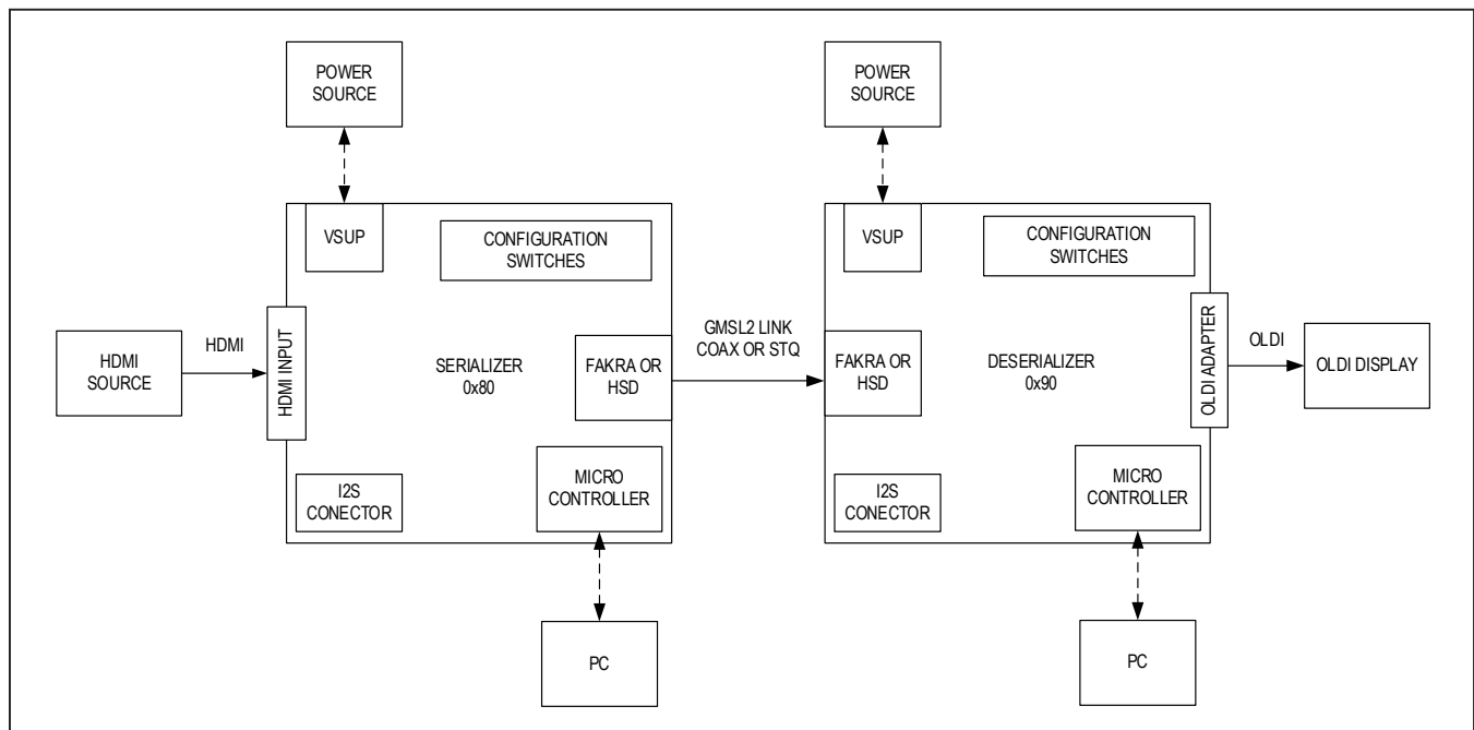
Figure 2. Typical GMSL System Evaluation Setup Block Diagram
