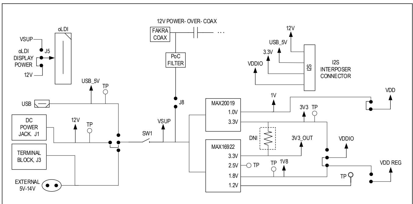
Figure 4. Deserializer Evaluation Board Power Block Diagram
