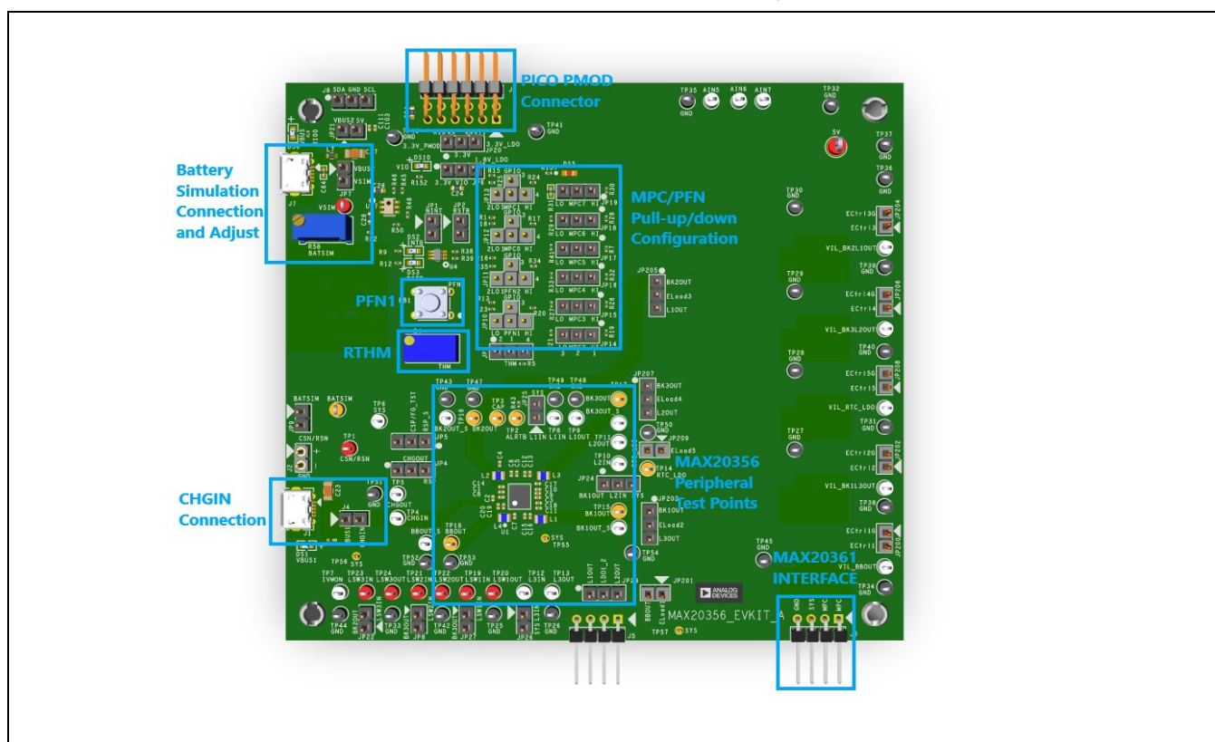
Figure 14. MAX20356 EV Kit Block Annotated Picture
