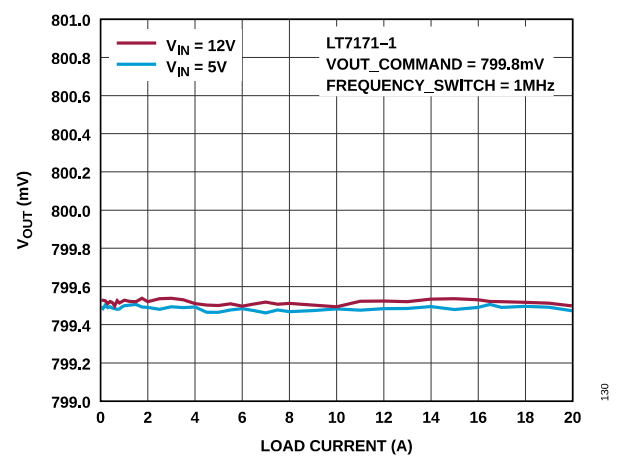
Figure 15. Load Regulation
