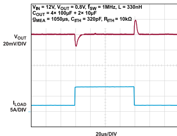
Figure 31. LT7171-1 Transient Response: Load Current Step, 2A to 8A
