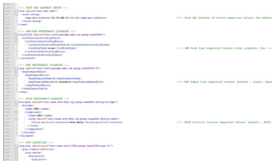
Figure 19. Device MAC Address, Redundancy Configuration, MSTP, PTP/PHY Latency
