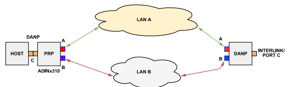
Figure 109. Example of Switch Configuration as PRP-DANP (Host Connected over Ethernet)
