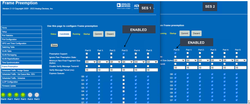
Figure 77. Candidate Page View to Enable and Configure Preemption
