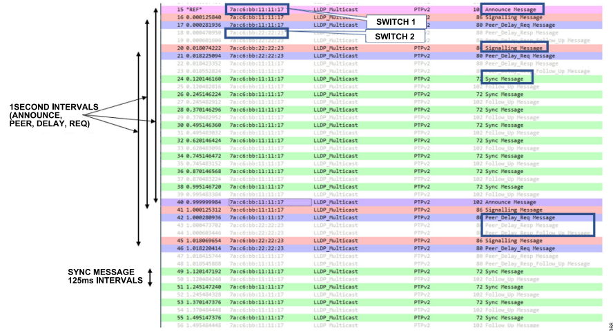
Figure 68. Time Synchronization View of Messaging through Wireshark Using an Ethernet Tap between Two Devices
