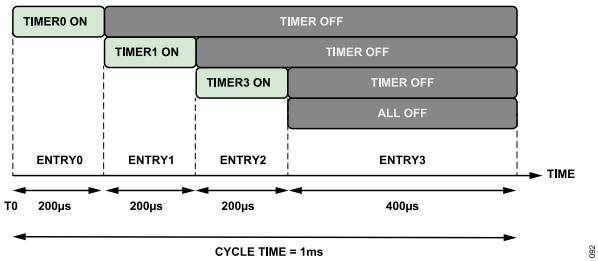
Figure 101. Schedule for Switch 1 Timer Pins
