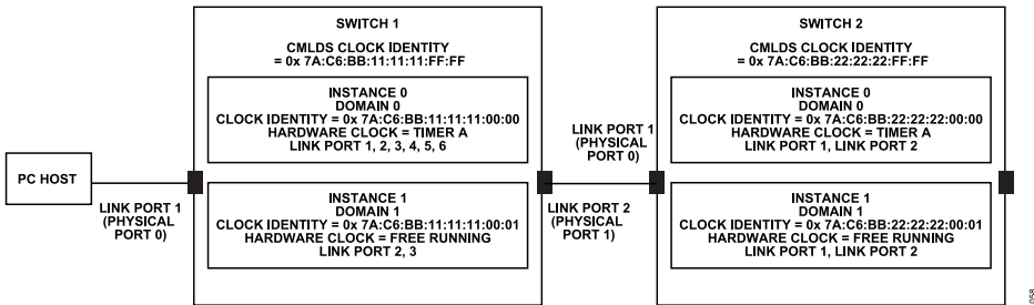
Figure 60. Time Synchronization with Two Instances
