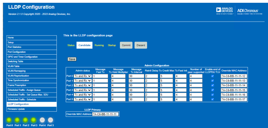
Figure 103. LLDP Candidate Page
