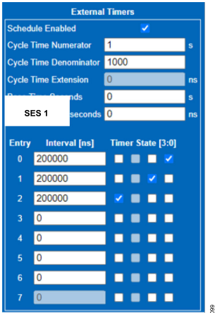
Figure 99. Configured Schedule for Switch 1 Timers
