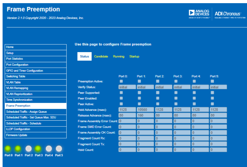
Figure 76. Frame Preemption Status Page
