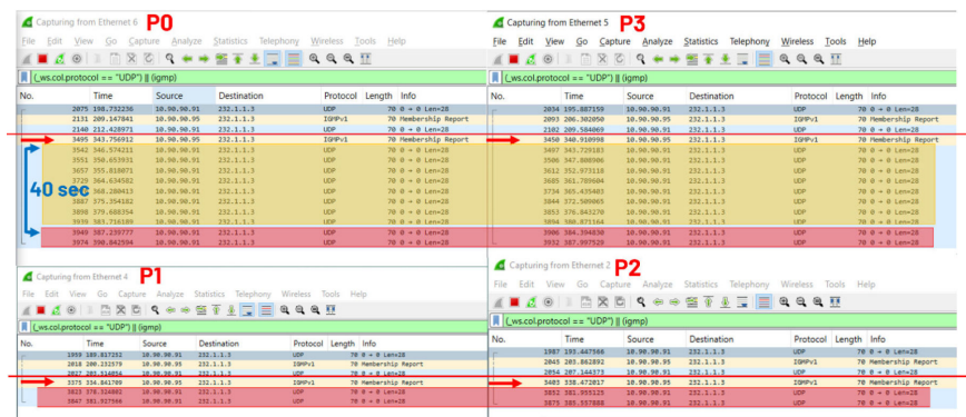
Figure 174. IGMPv1 Multicast Group Created and Group Member Timeout
