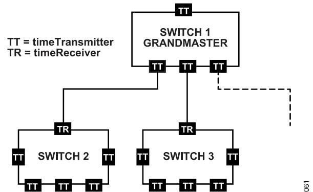
Figure 63. Time Synchronization Example for External Port Config
