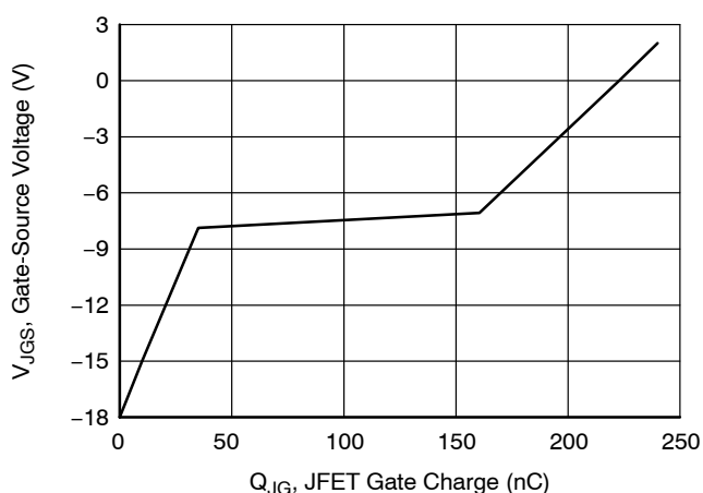
Figure 27. Typical JFET gate charge at V_{DS} = 400\text{ V} and I_D = 60\text{ A}
