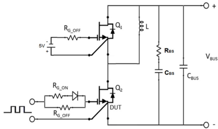
Figure 23. Schematic of the Half-Bridge Mode Switching Test Circuit. Note, a Bus RC Snubber ( R_{BS} = 2.5\ \Omega , C_{BS} = 200\ \text{nF} ) is Used to Reduce the Power Loop High Frequency Oscillations
