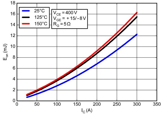
Figure 50. Typical Switching Energy Eon vs. IC
