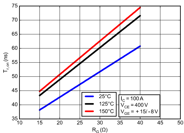
Figure 37. Typical Switching Time Tron vs. RG
