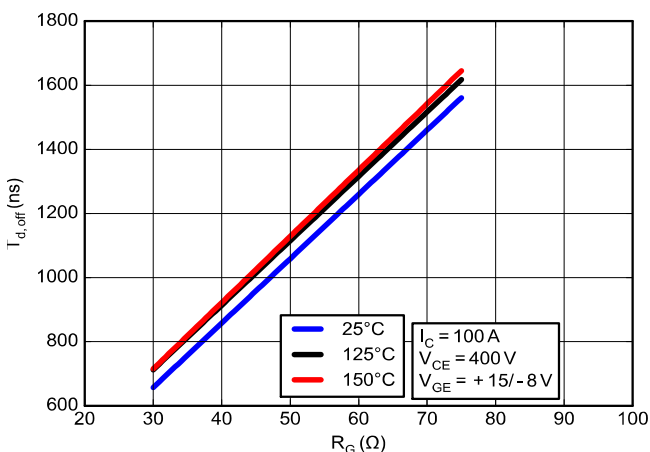
Figure 35. Typical Switching Time Tdoff vs. RG
