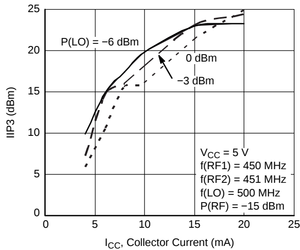
Figure 6. IIP3 - I_{CC}
