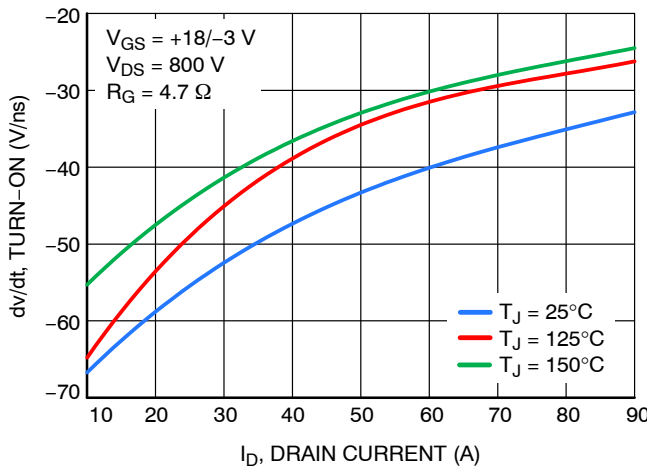
Figure 21. dv/dt Turn ON vs. Drain Current V_{DS} = 800 \text{ V}
