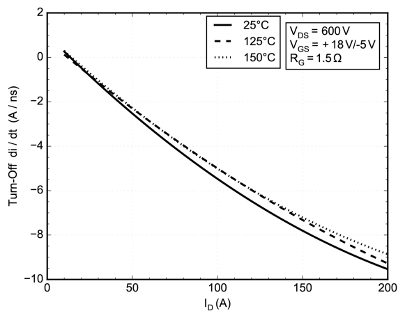
Figure 23. di/dt OFF vs I_D
