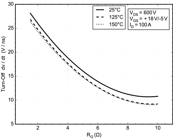
Figure 28. dv/dt OFF vs. R_G
