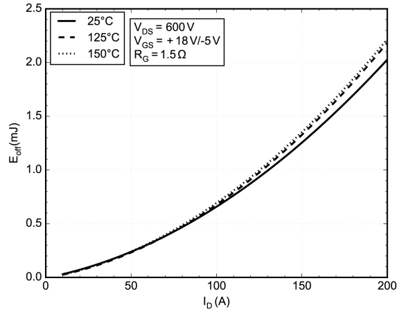
Figure 11. Typical Switching Loss E_{off} vs. I_D
