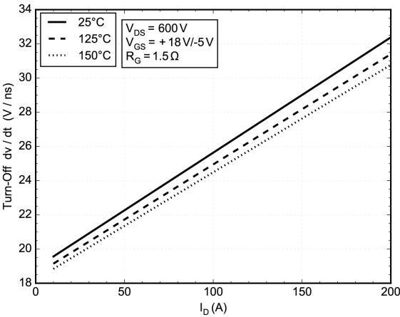
Figure 27. dv/dt OFF vs I_D
