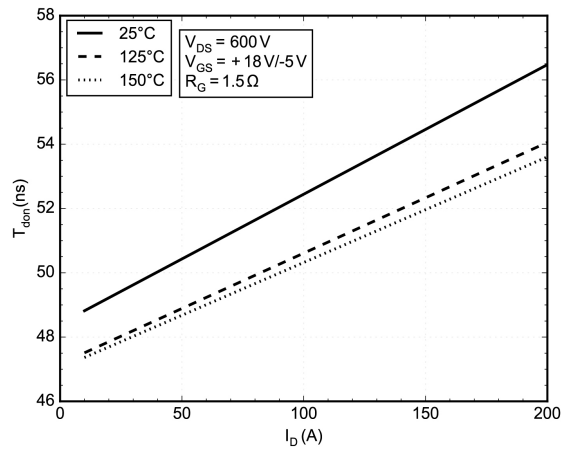
Figure 13. Typical Turn-On Switching T_{d(on)} vs. I_D
