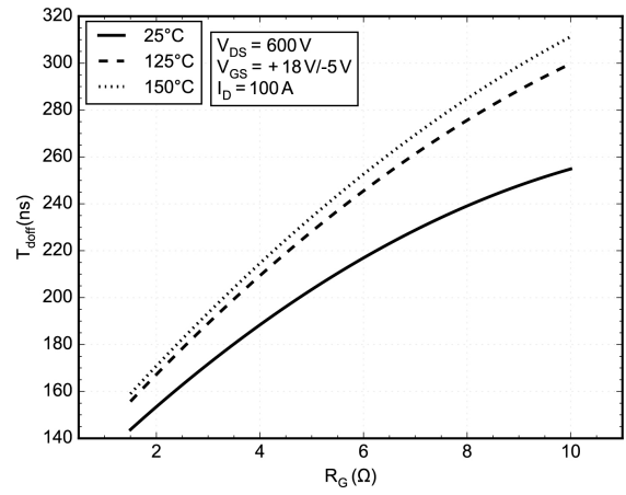
Figure 16. Typical Turn-off Switching T_{d(off)} vs. R_G
