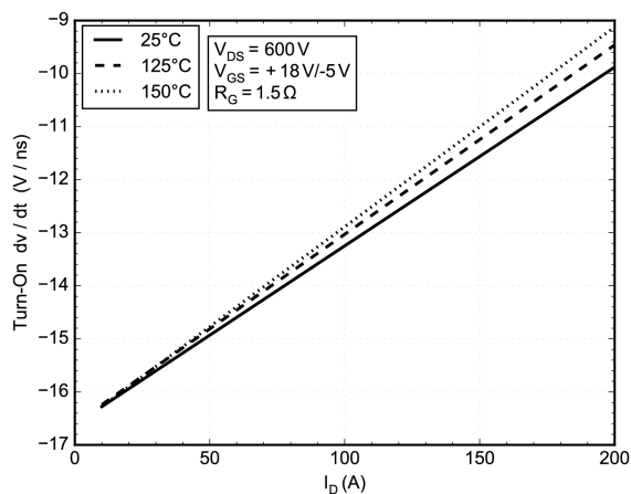
Figure 25. dv/dt ON vs I_D
