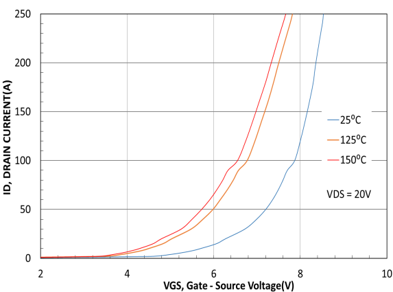
Figure 5. MOSFET Typical Transfer Characteristics
