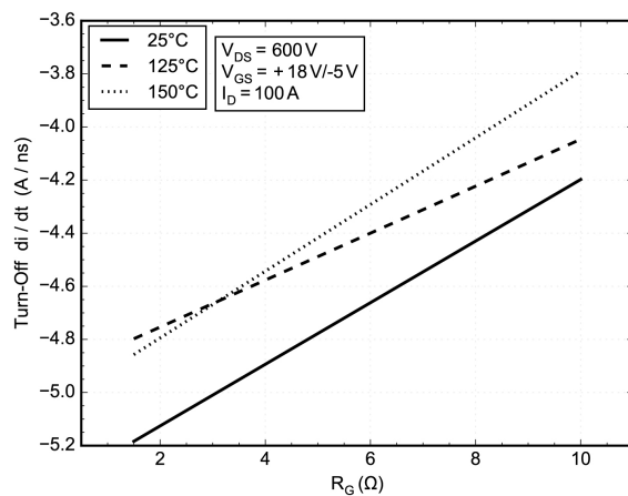
Figure 24. di/dt OFF vs R_G
