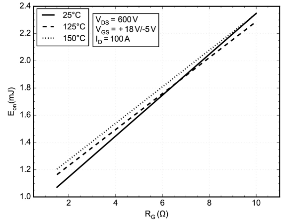
Figure 10. Typical Switching Loss E_{on} vs. R_G
