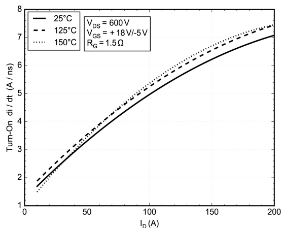
Figure 21. di/dt ON vs I_D
