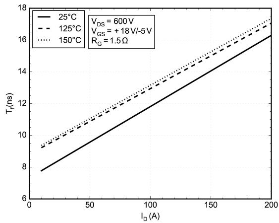
Figure 19. Typical Turn-Off Switching T_f vs. I_D
