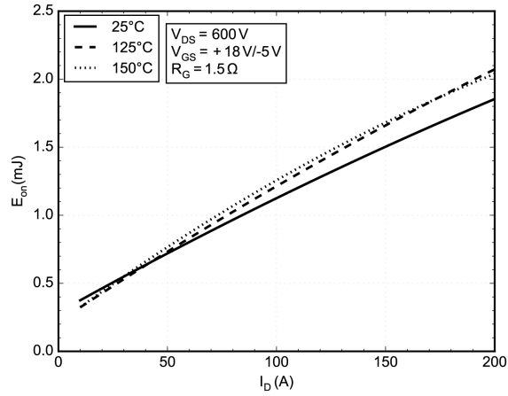
Figure 9. Typical Switching Loss E_{on} vs. I_D
