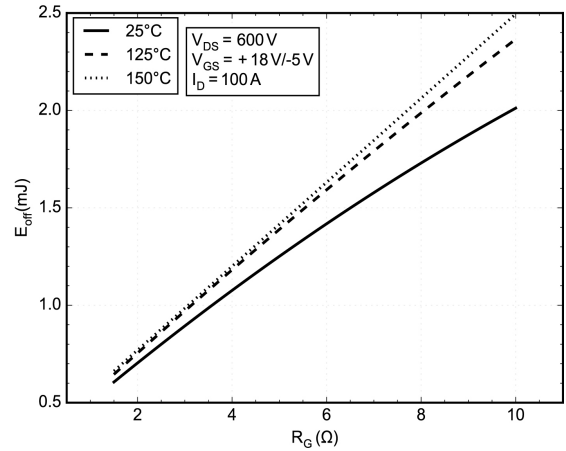
Figure 12. Typical Switching Loss E_{off} vs. R_G
