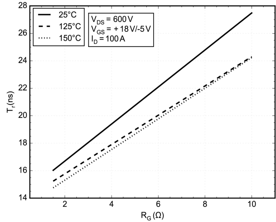
Figure 18. Typical Turn-On Switching T_r vs. R_G
