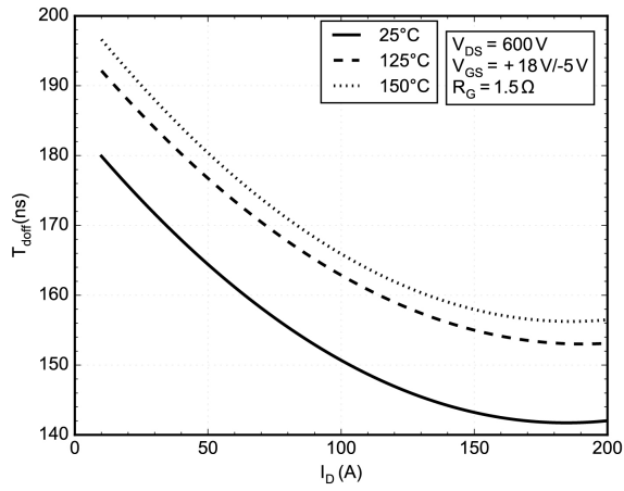
Figure 15. Typical Turn-off Switching T_{d(off)} vs. I_D
