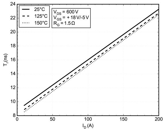
Figure 17. Typical Turn-On Switching T_r vs. I_D
