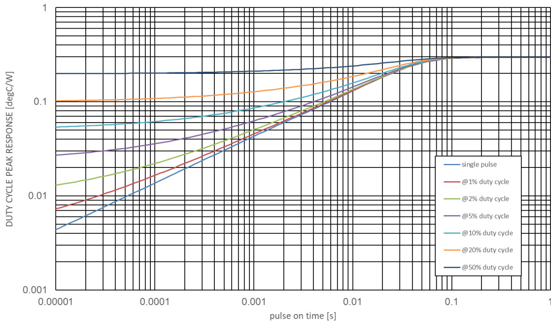
Figure 29. SiC MOSFET Junction-to-Case Transient Thermal Impedance
