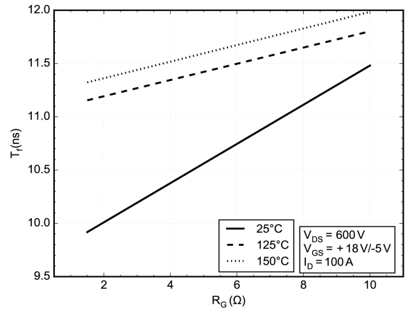
Figure 20. Typical Turn-Off Switching T_f vs. R_G
