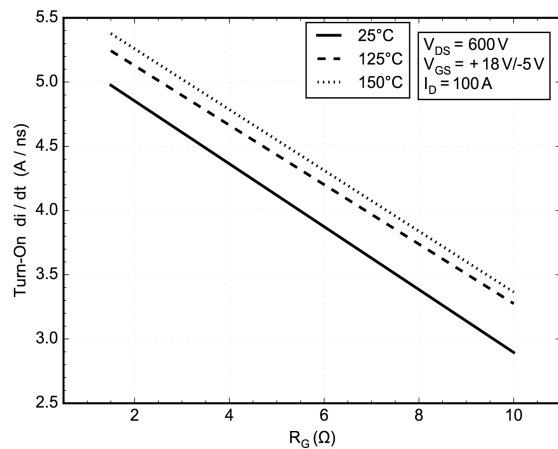
Figure 22. di/dt ON vs R_G
