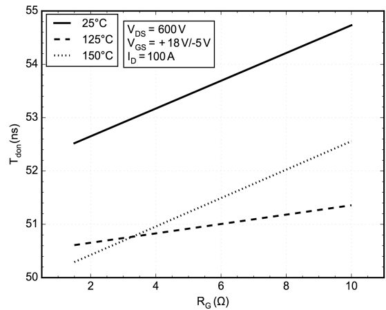
Figure 14. Typical Turn-On Switching T_{d(on)} vs. R_G
