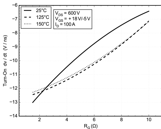
Figure 26. dv/dt ON vs R_G
