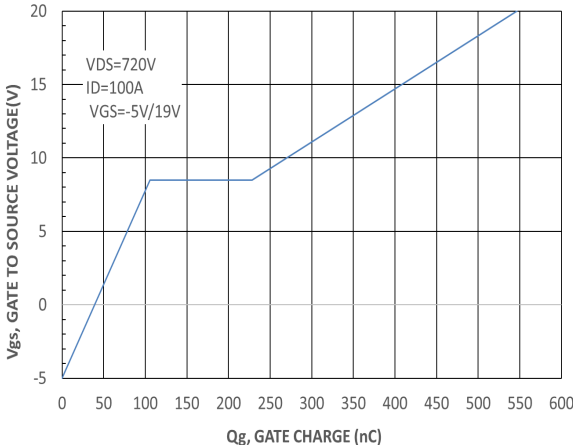
Figure 7. Gate-to-Source Voltage vs. Total Charge
