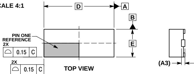
DFN16, 4x1.6, 0.5P CASE 506AC ISSUE D
