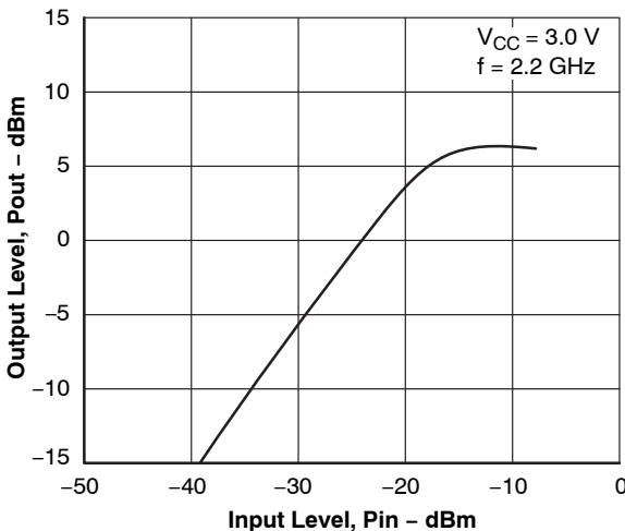
Figure 9. P_{out} - P_{in}
