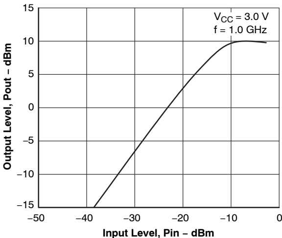
Figure 8. P_{out} - P_{in}
