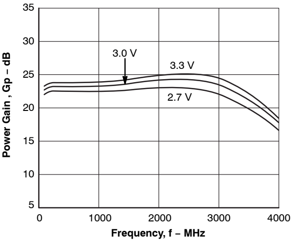
Figure 4. G_p - f
