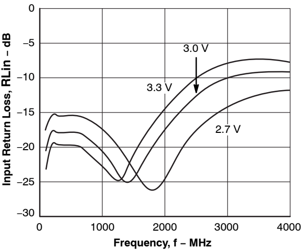
Figure 5. RL_{in} - f
