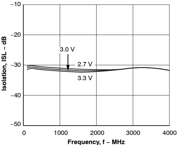
Figure 6. ISL - f
