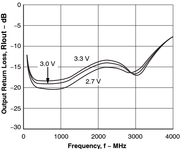
Figure 7. RL_{out} - f
