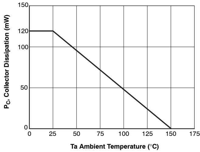
Figure 9. P_C - T_a
