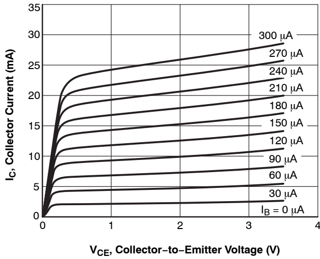
Figure 1. I_C - V_{CE}
