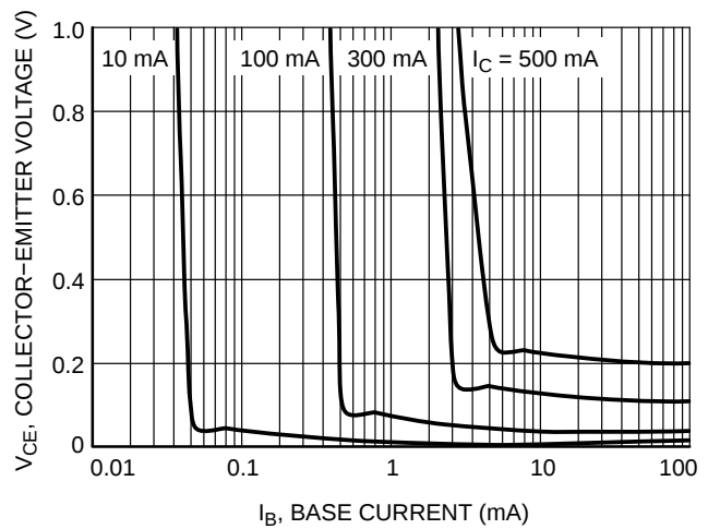
Figure 6. Saturation Region
