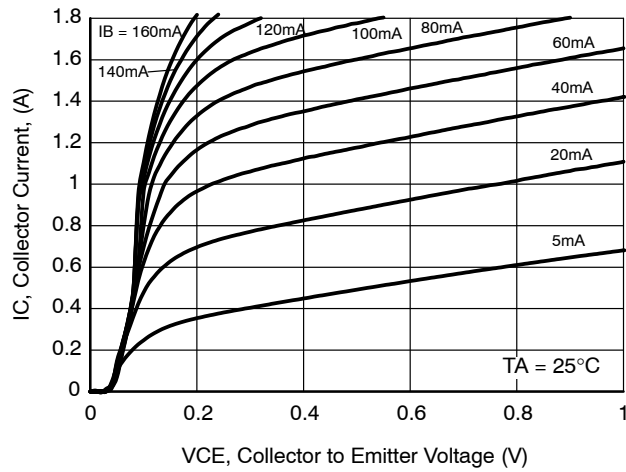
Figure 2. IC – VCE
