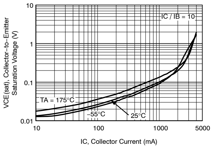
Figure 6. VCE(sat) – IC
