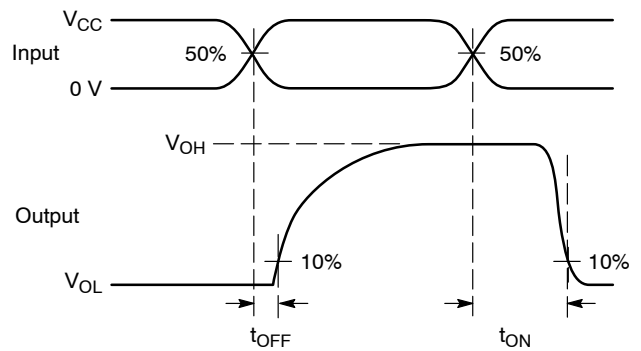
Figure 4. t_{ON}/t_{OFF}
