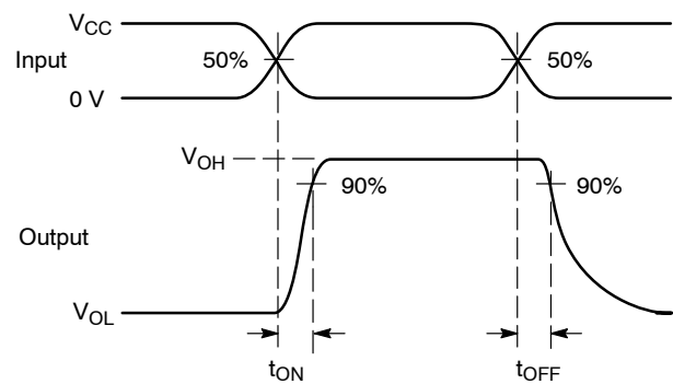
Figure 3. t_{ON}/t_{OFF}
