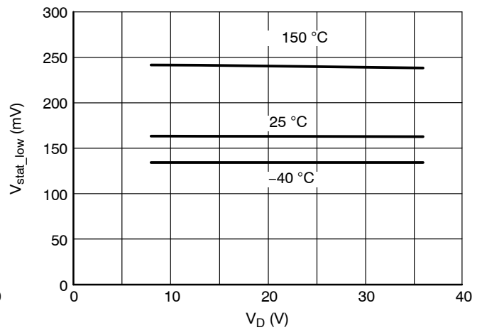
Figure 20. STAT Low Voltage vs. V_D
