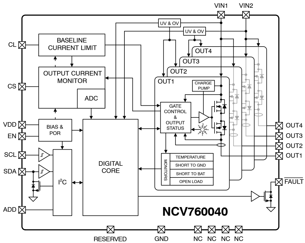
Figure 2. Block Diagram
