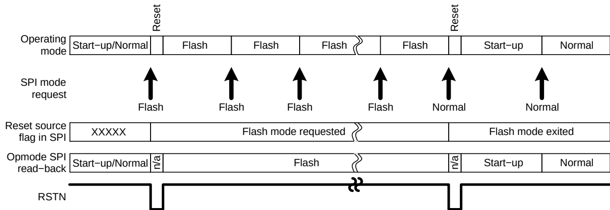
Figure 13. Flash Mode Sequence
