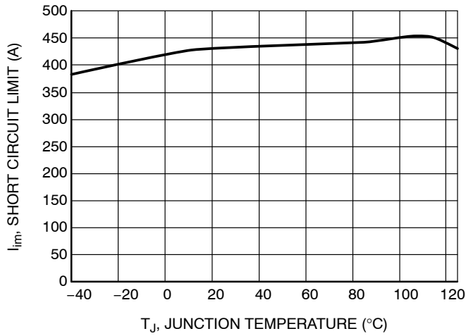
Figure 7. Short Circuit Current Limit vs. Temperature for V_{out1}
