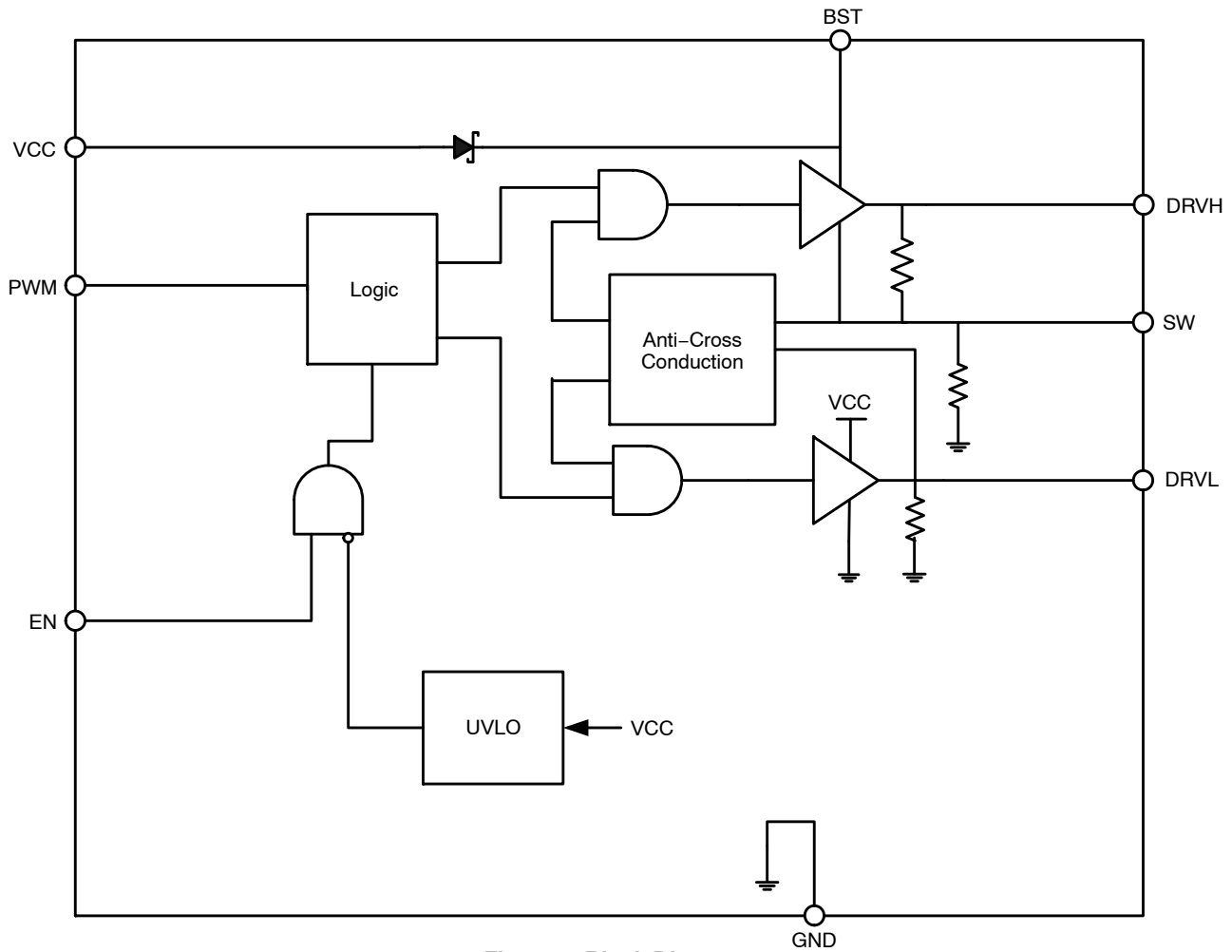
Figure 1. Block Diagram
