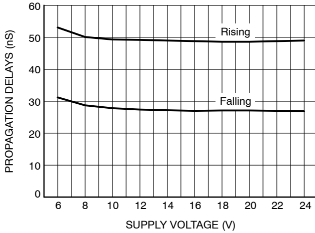
Figure 7. Propagation Delays vs. Supply Voltage
