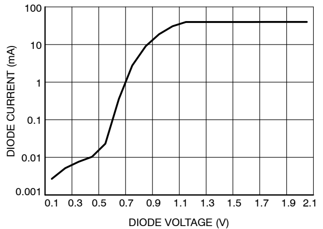
Figure 12. Diode Current vs. Diode Voltage
