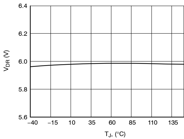
Figure 18. V_{DR} Driver Voltage vs. Temperature, I_N = 0 , R_{ON} = 0 , External Load 10 mA
