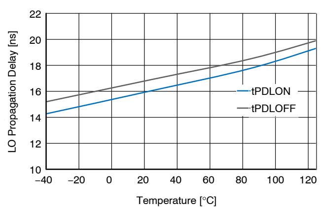
Figure 14. LIN to LOSRC Propagation Delay vs. Temperature
