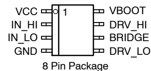
8 Pin Package
