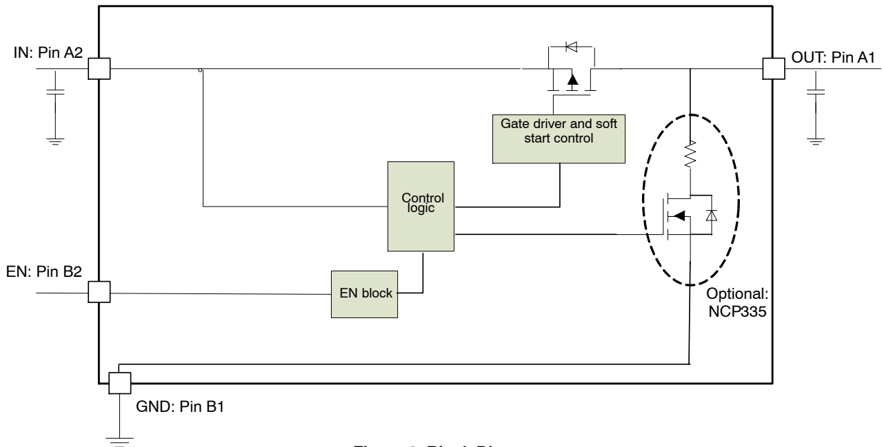
Figure 2. Block Diagram
