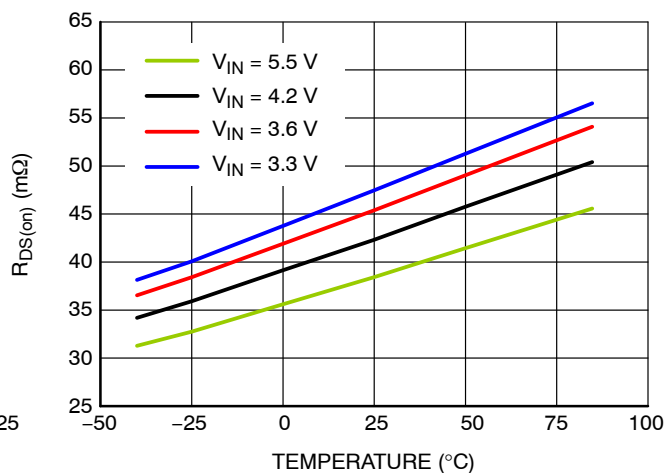
Figure 7. R_{DS(on)} ( m\Omega ) vs. Temperature ( ^{\circ}C ), I_{LOAD} 2 A
