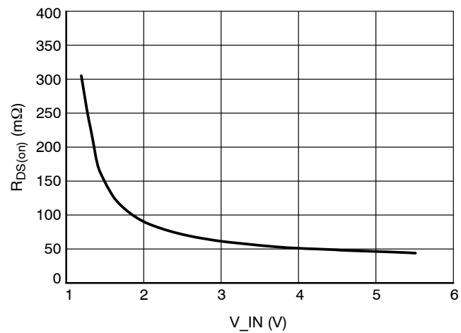
Figure 4. R_{DS(on)} ( m\Omega ) vs. V_{IN} (V) ( I_{LOAD} = 100 mA & Temp 25°C)
