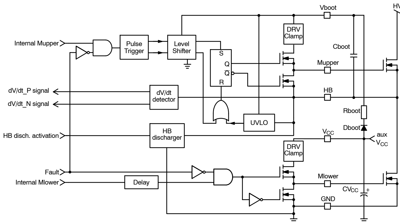
Figure 50. The NCP13994 Internal DRV Structure
