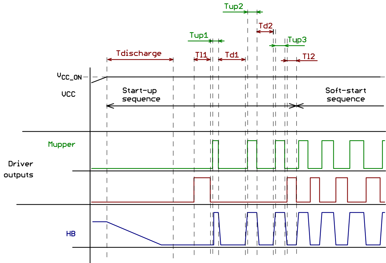
Figure 43. Dedicated Startup Sequence Detail
