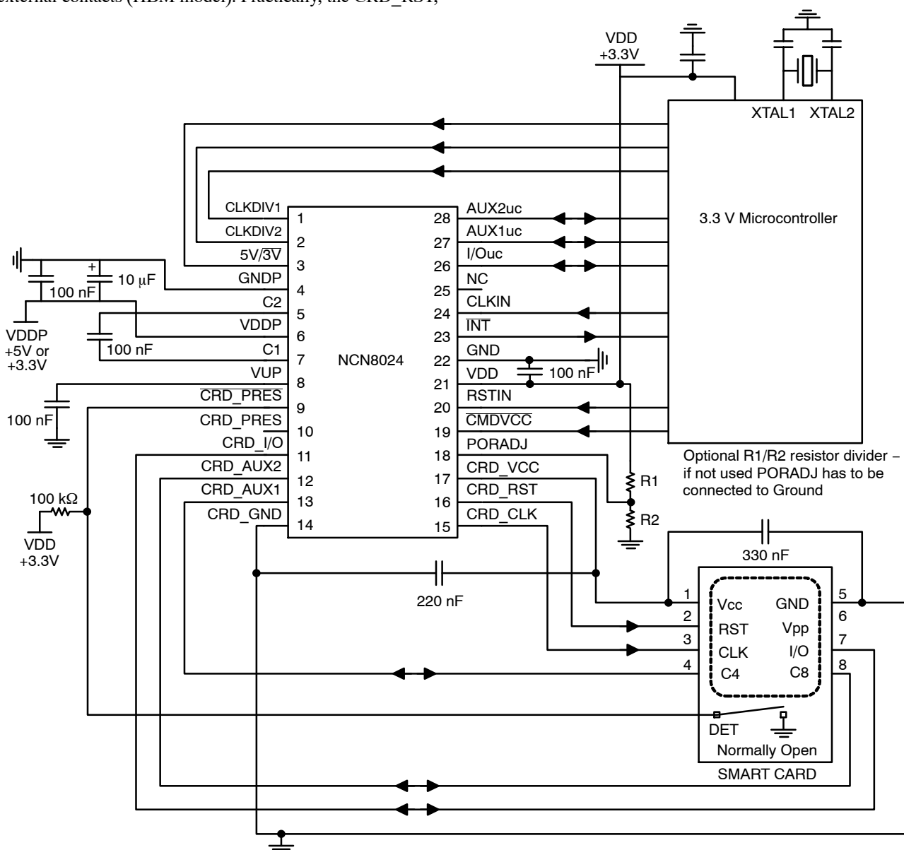
Figure 8. Application Schematic
