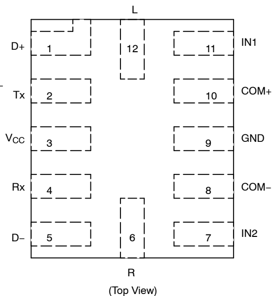
Figure 2. Pinout Diagram
