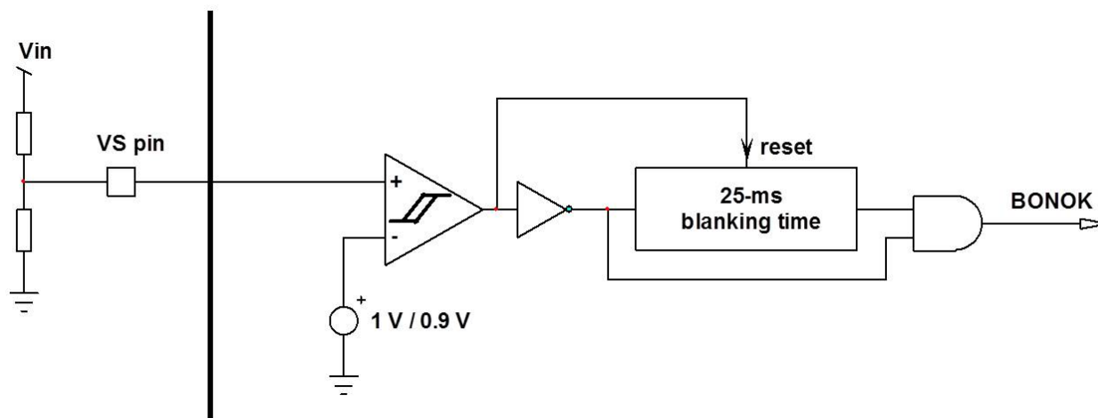
Figure 69. Brown-out Circuit
