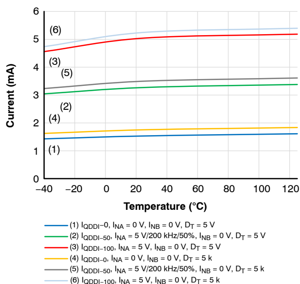
Figure 14. I_{QDDI} Supply Current, V_{DDI} = 5 V
