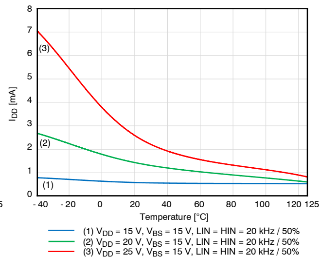
Figure 11. I_{DD} Supply Current V_{DD} = 15\text{--}25\text{ V} , LIN = HIN = 20 kHz / 50%
