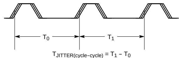
Figure 9. Cycle-to-Cycle Jitter
