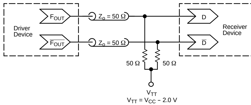
Figure 14. Typical Termination for Output Driver and Device Evaluation (See Application Note AND8020/D – Termination of ECL Logic Devices.)
