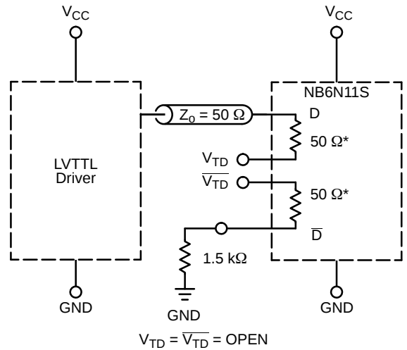
Figure 16. LVTTTL Interface
