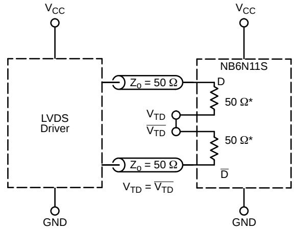
Figure 12. LVDS Interface
