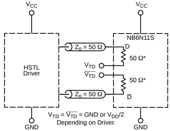
Figure 14. HSTL Interface
