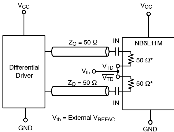
Figure 13. Capacitor-Coupled Differential Interface ( V_{TD}/\bar{V}_{TD} Connected to V_{REFAC} ; V_{REFAC} Bypassed to Ground with 0.1 \mu F Capacitor)
