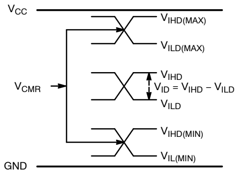
Figure 8. V_{CMR} Diagram
