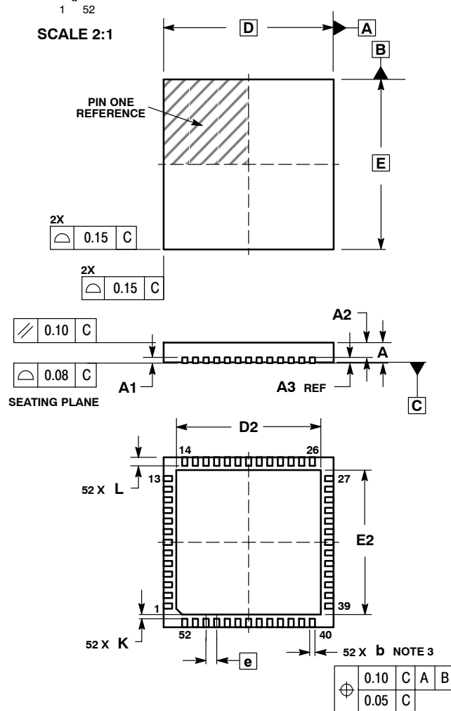
QFN52 8x8, 0.5P CASE 485M ISSUE C
