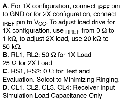
Figure 9. Typical Termination Configuration for Output Driver and Device Evaluation C_{Lx} for Test Only (Representing Receiver Input Loading); Not Added to Application
