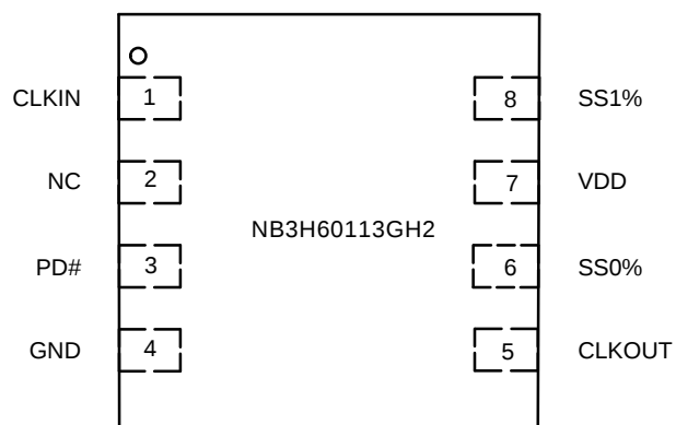
Figure 2. Pin Connections (Top View) – WDFN8
