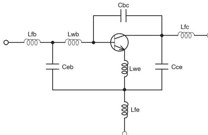
Figure 10. Schematic
