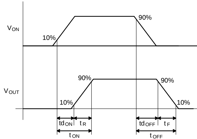
Figure 5. Timing Diagram
